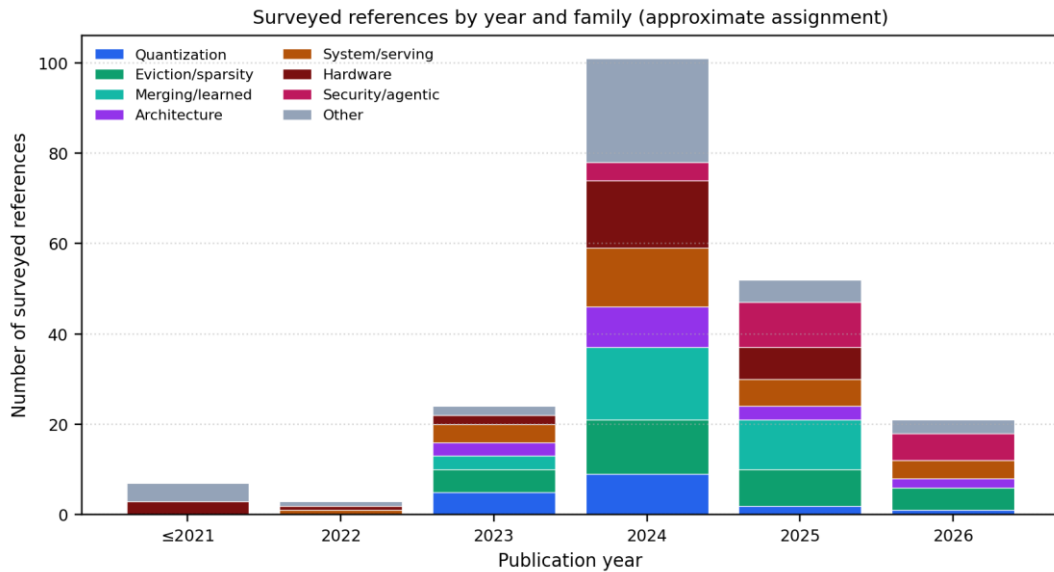
Fig. 3. Surveyed references by publication year and method family (approximate single-family assignment from the reference corpus). Takeaway: the field expanded sharply in 2024 and stays active into 2025-2026, and the security and agentic categories appear only in the latest years, marking them as emerging and under-surveyed.
